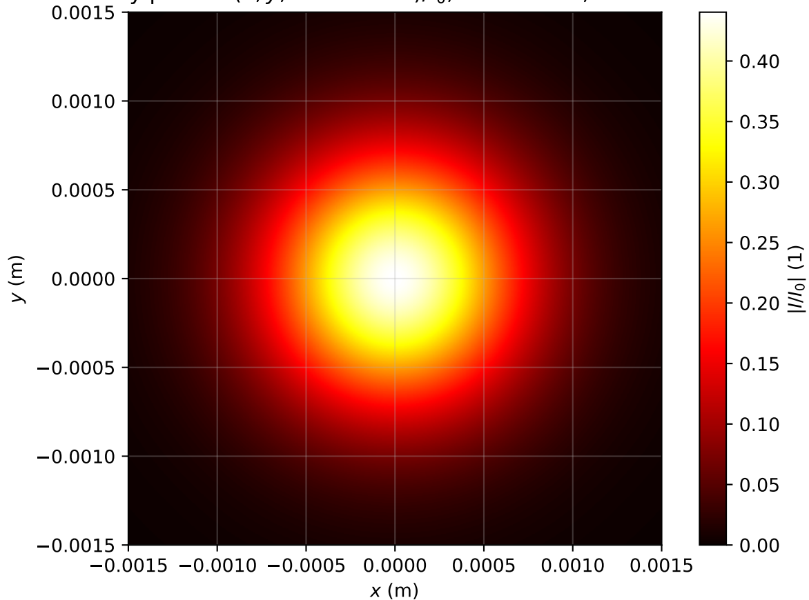
Intensity profile I(x, y, z = 3.662m)/I_0 , P_{in}=0.5P_{cr} , artificial time
